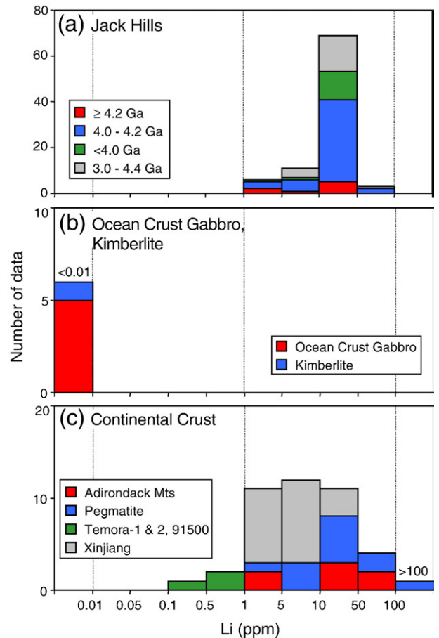
Fig. 4. Li abundance (ppm) of (a) Jack Hills zircons; (b) Ocean crust gabbro and Kimberlite zircons; (c) Continental crust zircons from Adirondack Mountains, pegmatites, Temora-1, Temora-2, 91500, and Xinjiang measured by an ion microprobe (Table 1, and Table S2 and S3 in the Supplementary Information).
